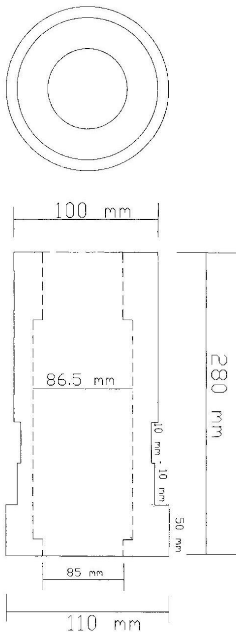
COOLING WATER PUMP SHAFT SLEEVE
