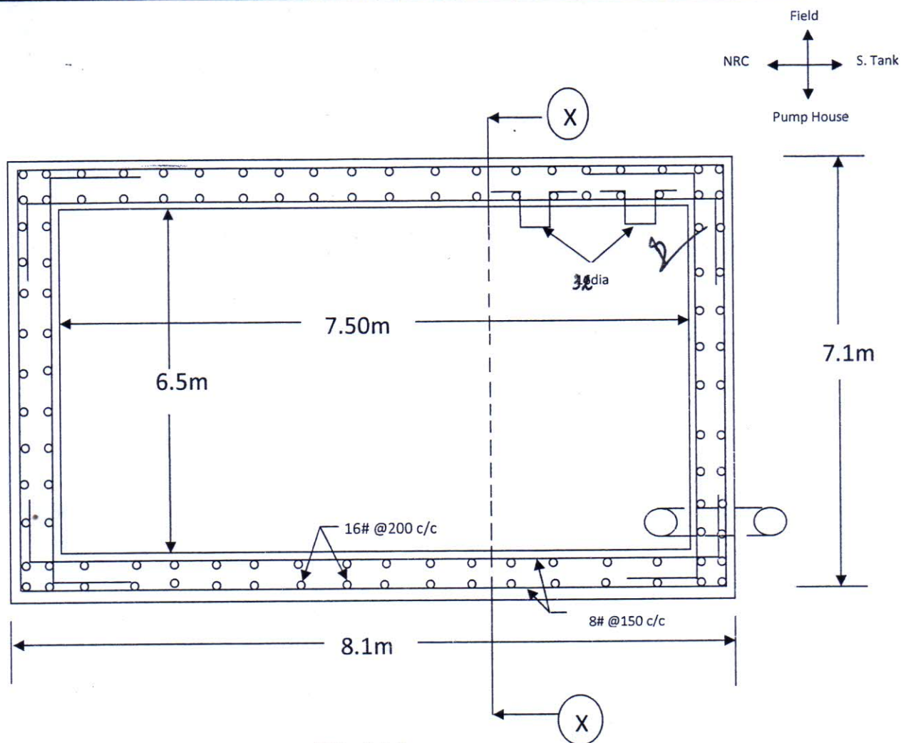
PLAN
