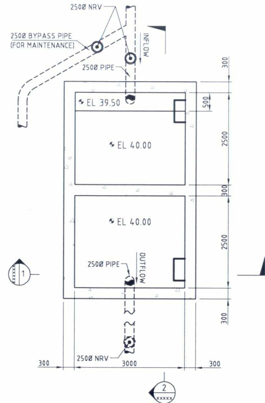
BOTTOM PLAN - EFFLUENT TANK SCALE (A1) 1:50
