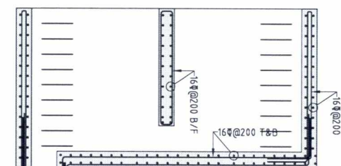
SECTION 4 SCALE (A1) 1:50
