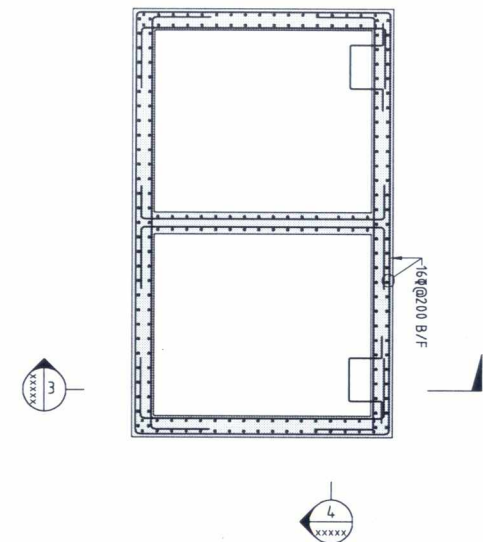
REINFORCEMENT TOP PLAN - EFFLUENT TANK SCALE (A1) 1:50
