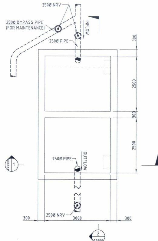
TOP PLAN - EFFLUENT TANK SCALE (A1) 1:50
