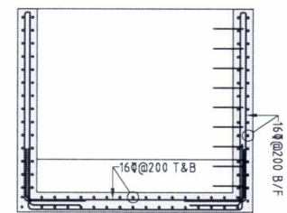
SECTION 3 SCALE (A1) 1:50
