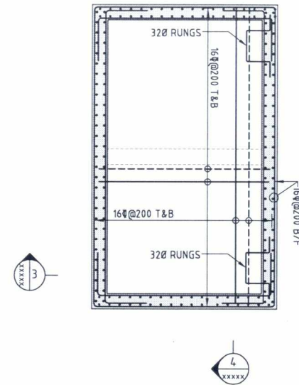
REINFORCEMENT BOTTOM PLAN - EFFLUENT TANK SCALE (A1) 1:50
